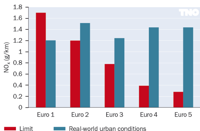
Figure 3. \text{NO}_x emissions of light commercial vehicles (vans) in urban conditions, compared to the emissions limit.
